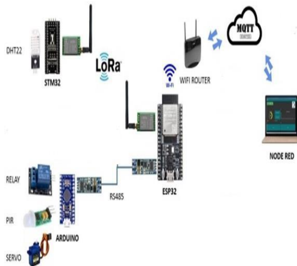
Figure 2. System Implementation
