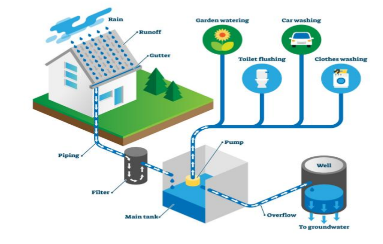
Figure 1. Rain Water Harvesting
